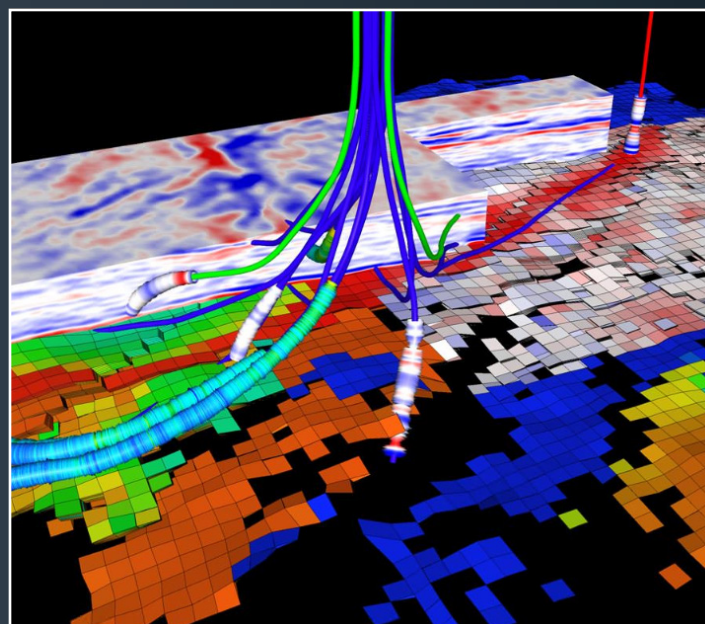
A quantitative analysis of temporal and spatial well data integrated with a dynamic reservoir simulation and 4D seismic data within a multidisciplinary data fusion environment.
