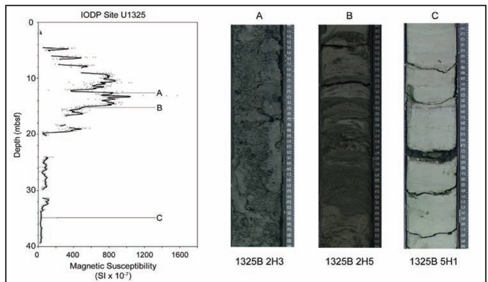
Figure 4: MS record at Site U1325 Hole B, offshore Vancouver Island and selected core photos. (A) Thick, massive sand turbidite and (B) thin turbidite sand beds correlate with high MS values. (C) Hemipelagic clay dominated interval that corresponds with low MS.
