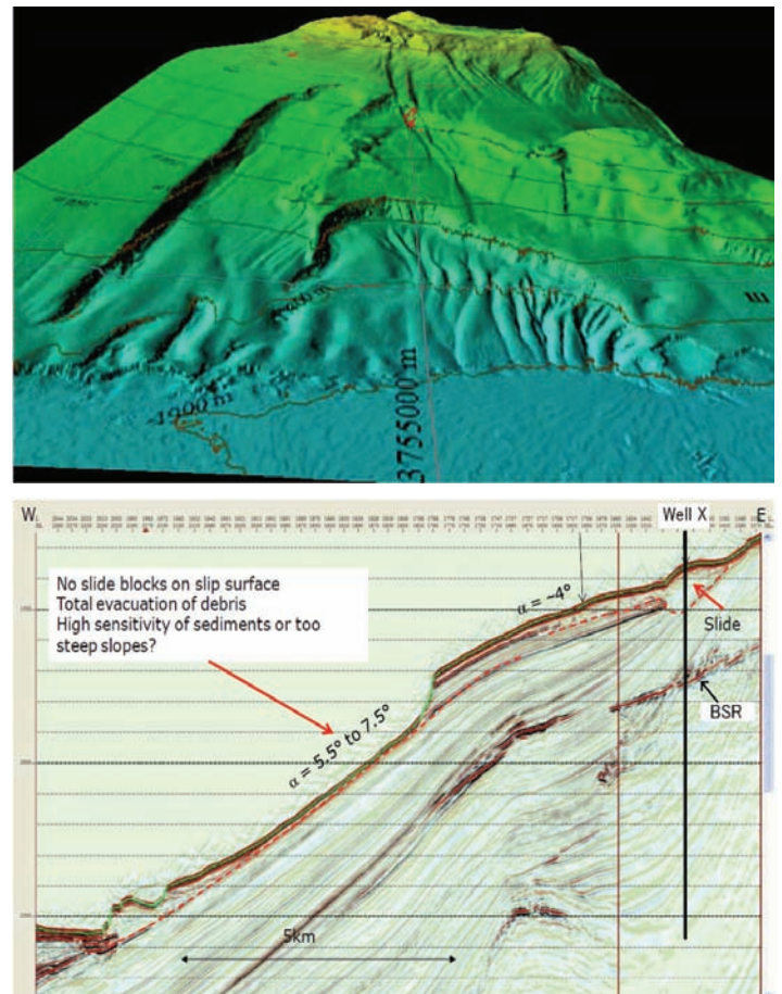
Figure 6: Landslide scars in the eastern Nankai Trough
