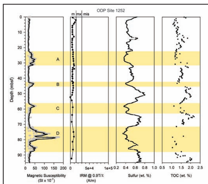
Figure 3: Down core measurements of MS, IRM (isothermal remnant magnetization), bulk Sulfur from XRF (calibrated from unpublished S data courtesy of Ji-Hoon Kim, Oregon State University), and TOC (total organic carbon) for Site 1252 Hole A at Hydrate Ridge, offshore central Oregon. IRM data and interpreted magnetic mineralogy (M = magnetite, MX= mixed magnetite and magnetic iron sulfides, and MIS = magnetic iron sulfides) from Larrasoña et al. (2006). Notice the lack of MIS or MX mineralogy within the four high MS zones (A-D, marked in yellow) and the corresponding low sulfur and TOC contents. MS zone D is observed on the seismic data (Figure 2) as the chaotic wedge of sediments near the base of the slope basin sequence and contains both debris flow and silty clay deposits. MS zone A is equivalent to the thick, chaotic, seismic wedge cored at Site 1251 (Figure 2), where debris flows and sand and silt turbidites were recovered. MS zones B and C contain non-distinct cores of silty clay and clay, however, the MS, TOC, Sulfur, and magnetic mineralogy characteristics suggest these two zones are slope failure dominated as well.
