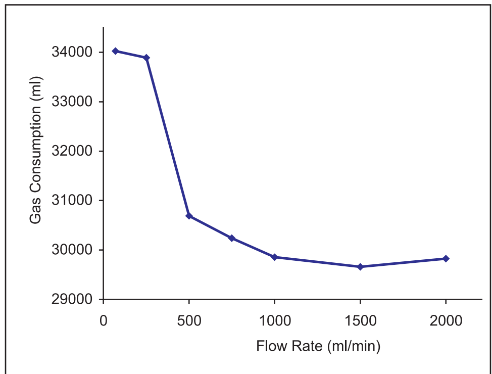
Figure 5. Hydrate gas consumption versus inlet gas flow rate in a depleted sediment (from Blake Ridge)/methane /water system.
