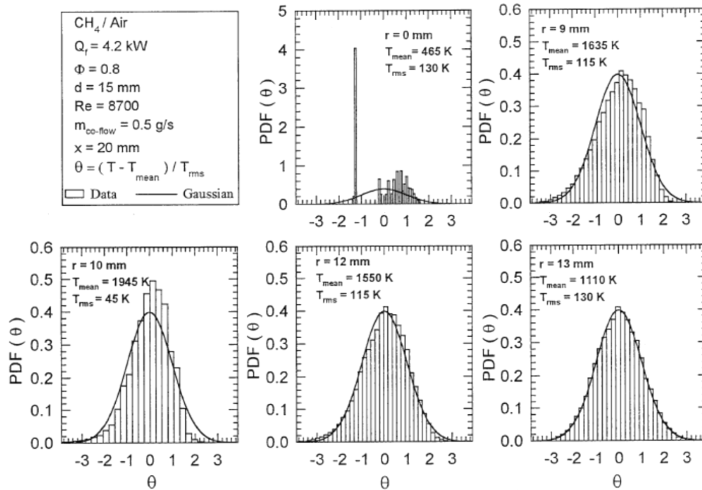
Figure 6.1 Normalized PDFs of temperature in \Phi = 0.8 , Q_f = 4.2 \text{ kW} flame at x = 20 \text{ mm}
