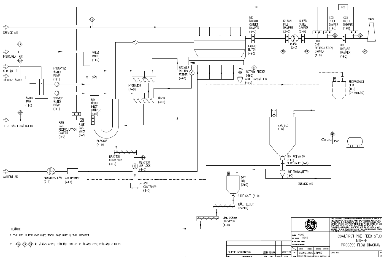
Figure 2-3 NID™ system Process Flow Diagram
