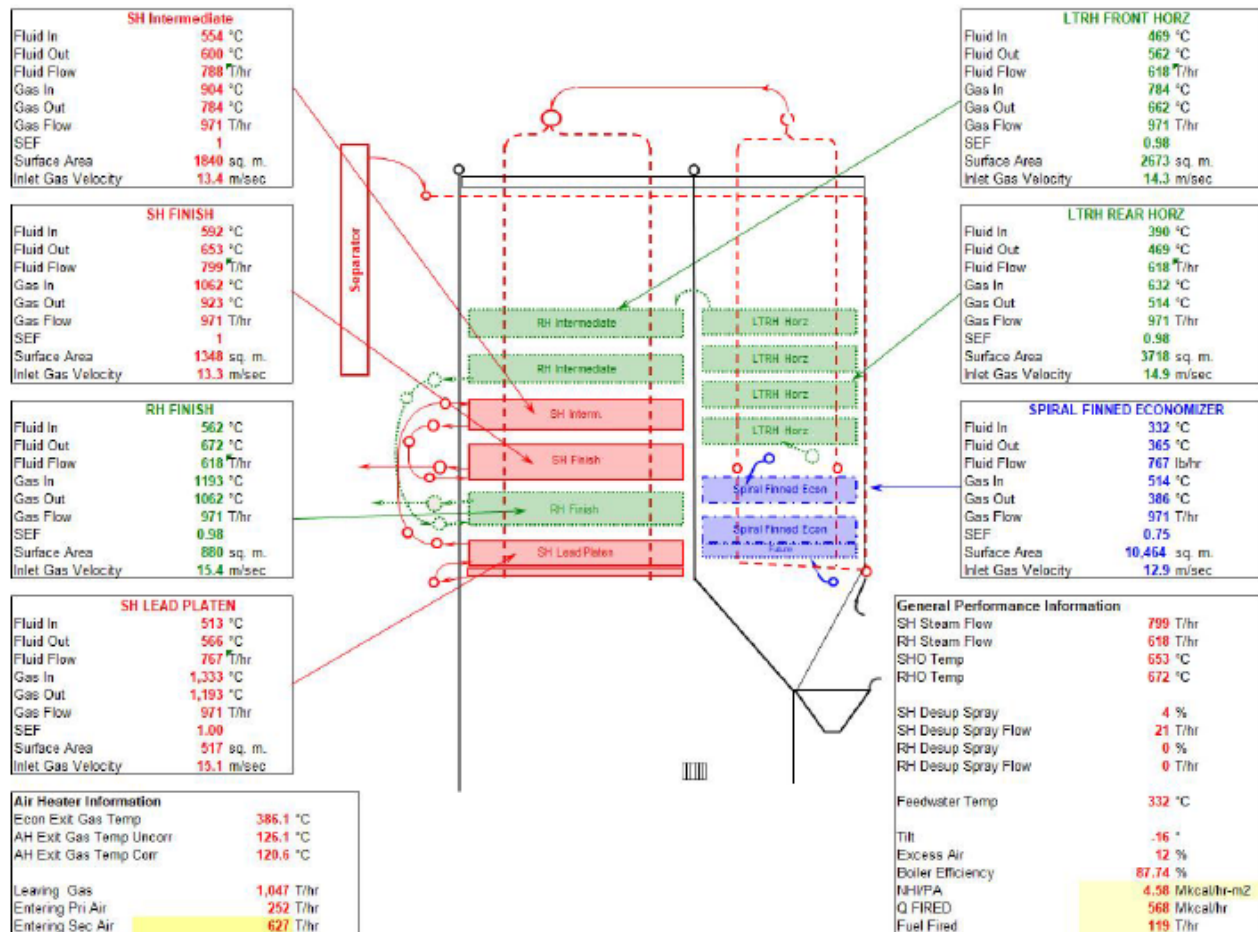
Figure 4-3 AUSC Boiler Expected Performance at VWO (103%) Load
